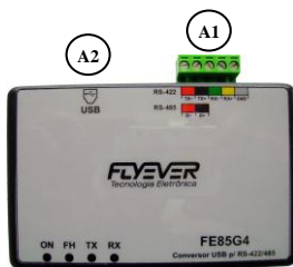
FE85G4 – Conversor USB/RS422.
